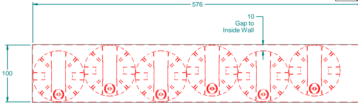
6 Tanks in 48' Dry Van
