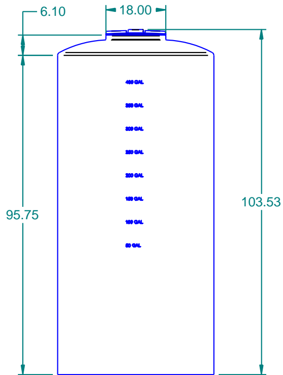
Side View
