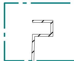
Typical Tank Lip Treatment SECTION A-A
