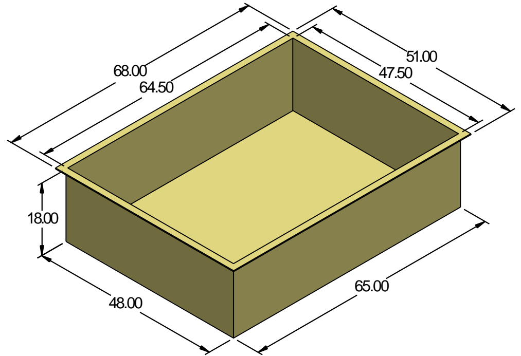
ISO View
