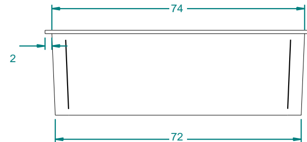
SECTION A-A Lip Treatment
