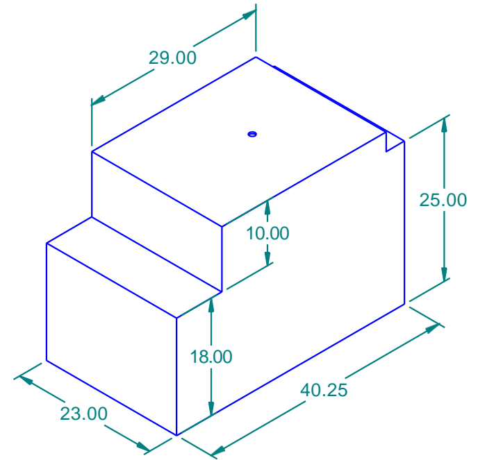
ISO View 300100
