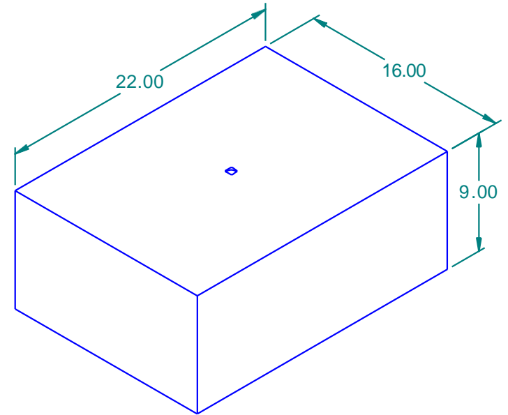
ISO View 120012
