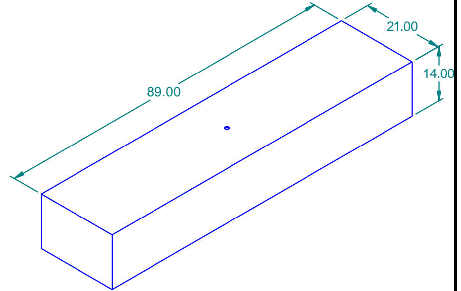
ISO View 103110
