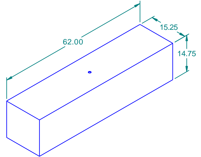
ISO View 103053
