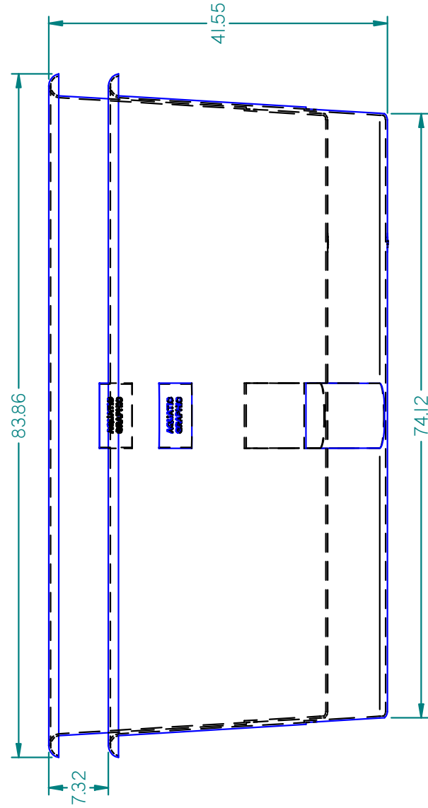
Nesting View
