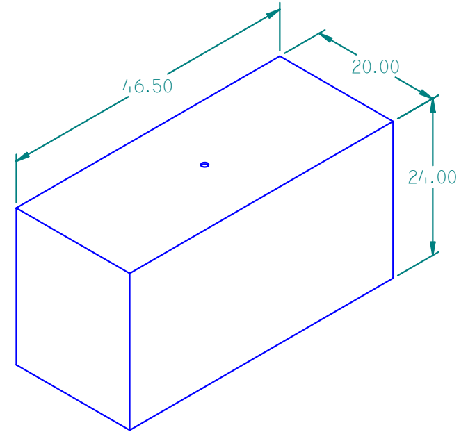
ISO VIEW 209090
