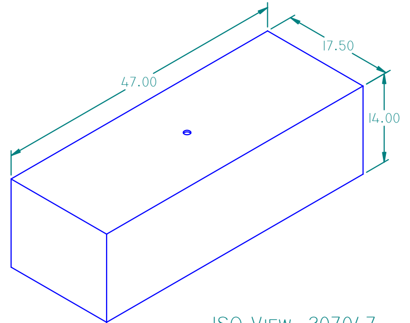
ISO VIEW 207047
