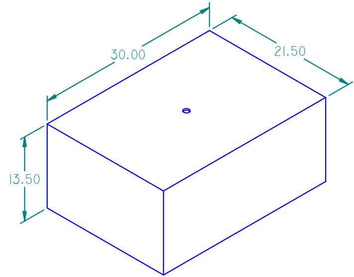
ISO VIEW 103040
