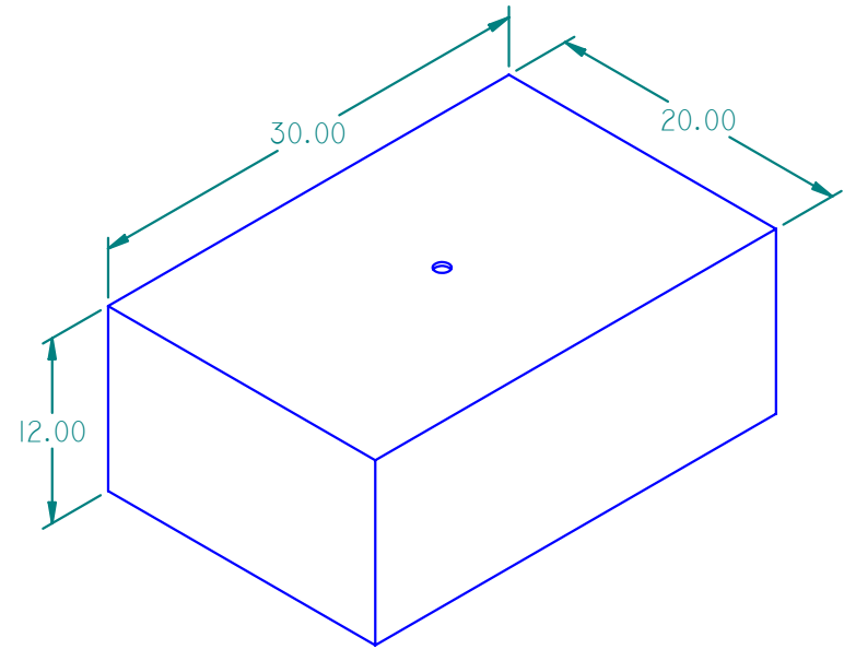
ISO VIEW 103030
