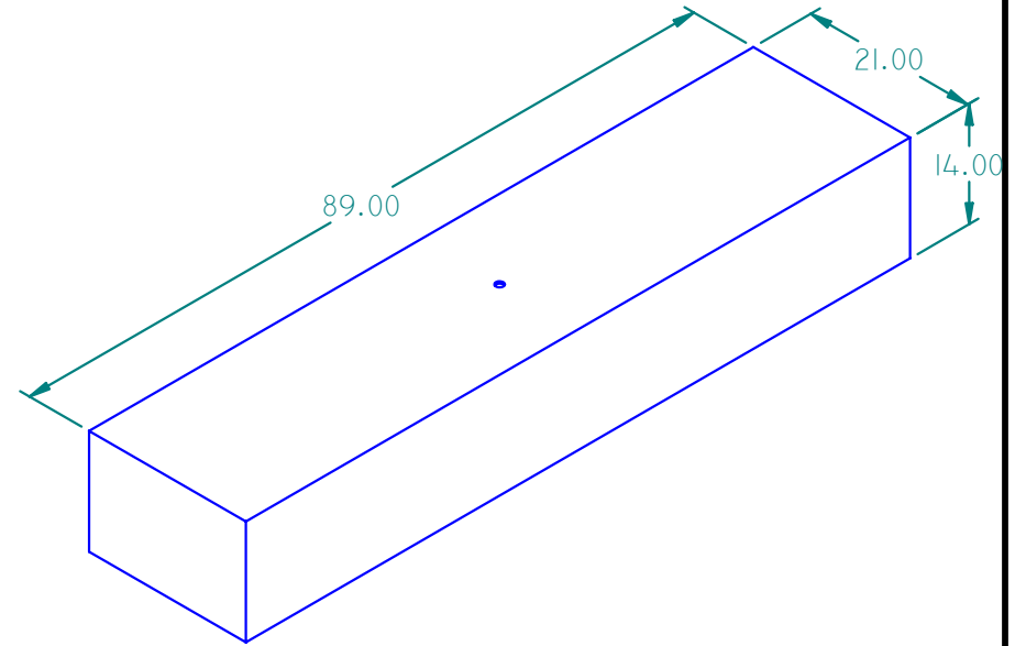
ISO VIEW 103110
